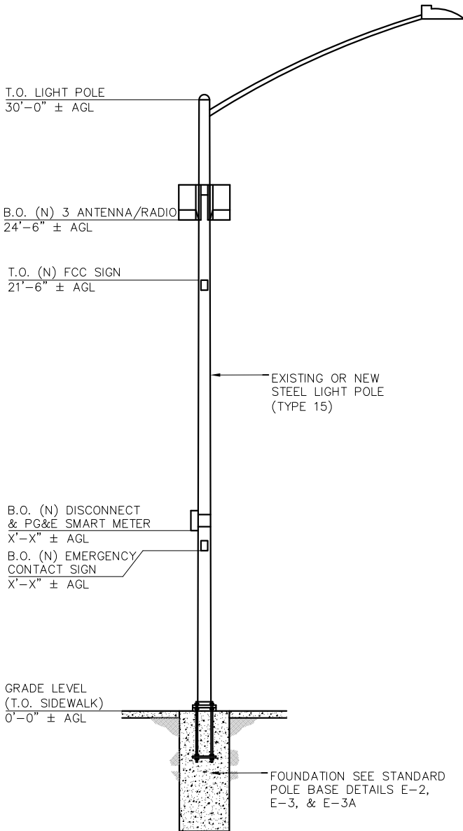
REPLACEMENT POLE ELEVATION VIEW
