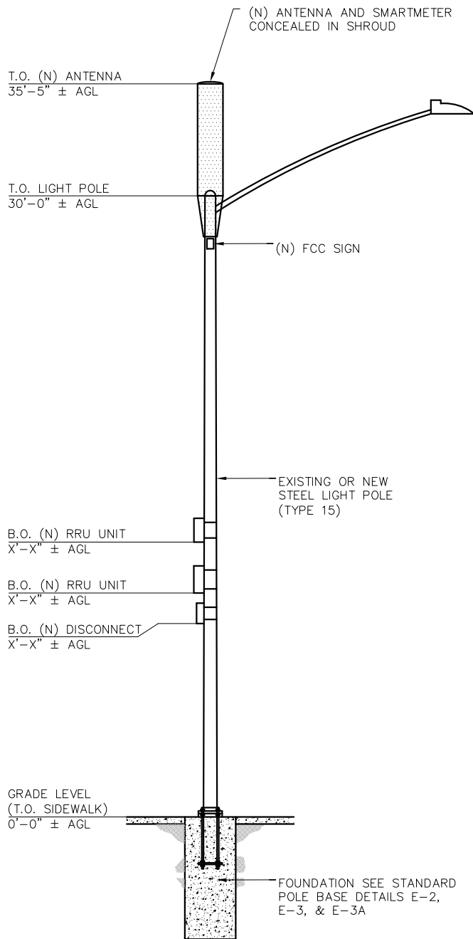
STACKED RRU UNIT (RETROFIT POLE) ELEVATION VIEW
